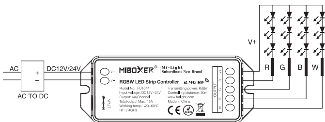
Controller connect to RGBW LED strip diagram
